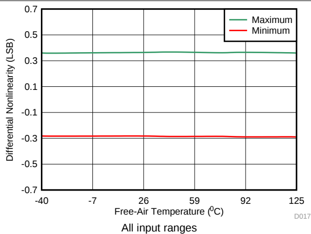
Figure 23. DNL vs Temperature
