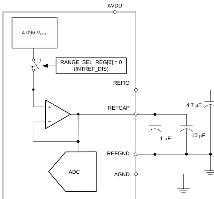
Figure 53. Device Connections for Using an Internal 4.096-V Reference
