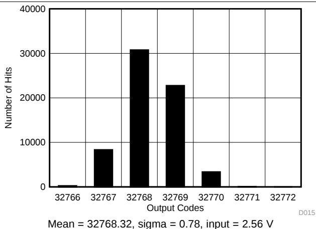
Figure 21. DC Histogram for Mid-Scale Inputs (0 V–5.12 V)
