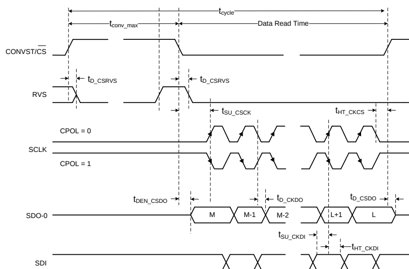
Figure 3. Standard SPI Interface Timing Diagram for \text{CPHA} = 0
