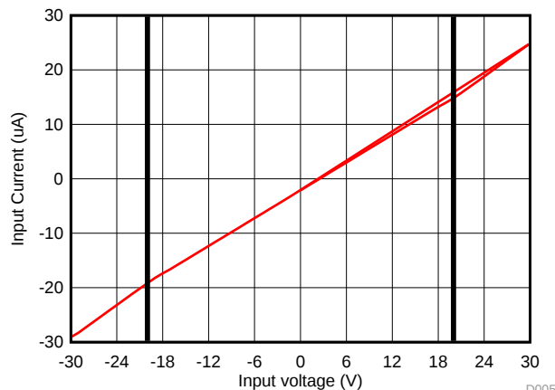
Figure 49. I-V Curve for the Input OVP Circuit (AVDD = 5\text{ V} )
