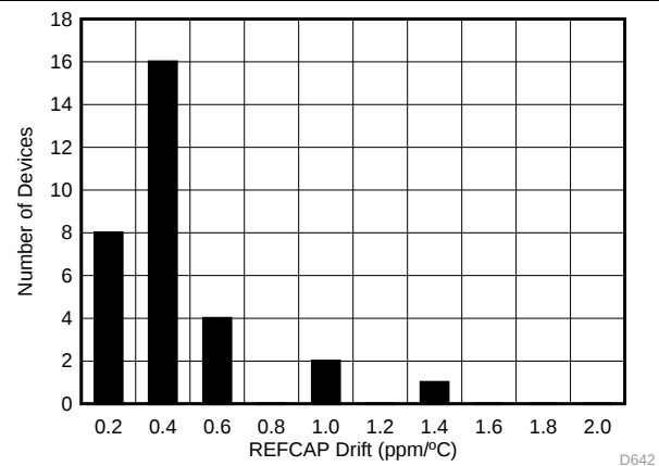
Figure 62. Reference Buffer Temperature Drift Histogram (PW Package)
