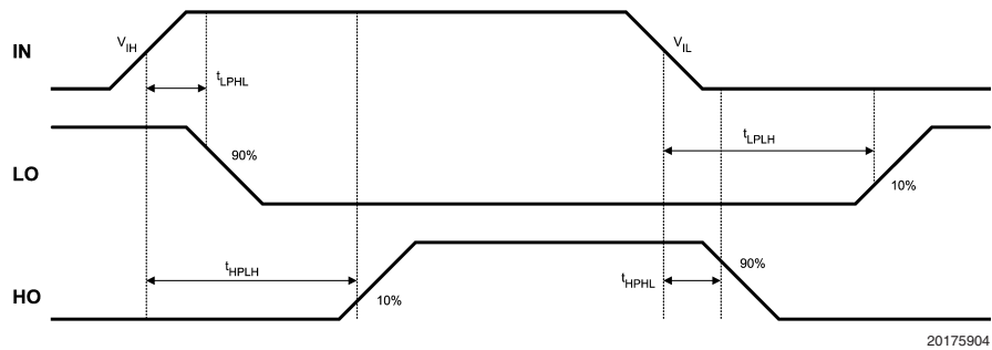
FIGURE 3. LM5106 Switching Time Definitions: t_{LPLH} , t_{LPHL} , t_{HPLH} , t_{HPHL}
