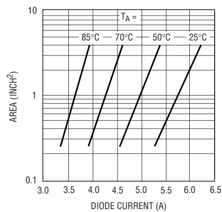
Figure 5. Maximum Diode Current vs PCB Area
