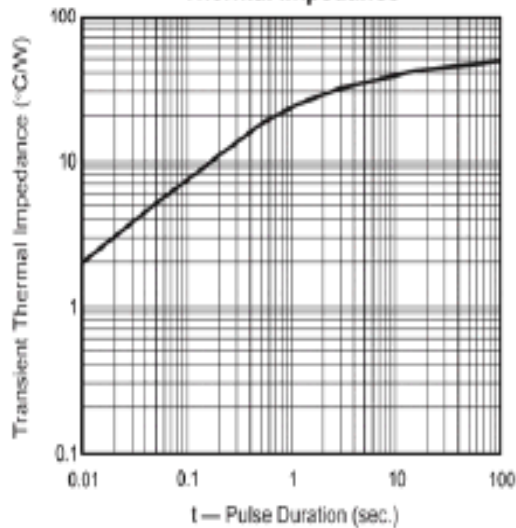
Fig. 6 - Typical Transient Thermal Impedance
