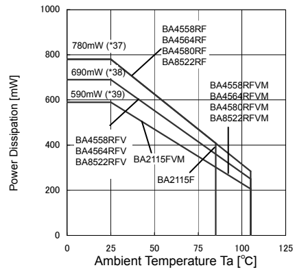
(c)BA4558R/BA4560R/BA4580R/BA8522R/BA2115 family
