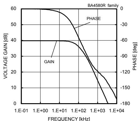
Fig. 132 Voltage Gain - Frequency ( V_{CC}/V_{EE}=+15[V]/-15[V] , A_v=40[dB] , R_L=2[k\Omega] , T_a=25[°C] )
