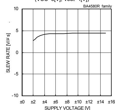
Fig. 128 Slew Rate - Supply Voltage ( C_L=100[pF] , R_L=2[k\Omega] , T_a=25[°C] )
