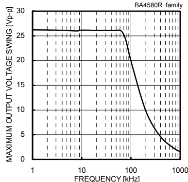
Fig. 131 Maximum Output Voltage Swing - Frequency ( V_{CC}/V_{EE}=+15[V]/-15[V] , R_L=2[k\Omega] , T_a=25[°C] )
