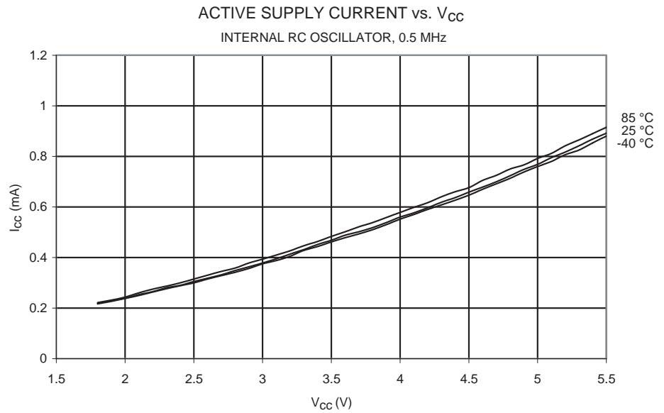
Figure 88. Active Supply Current vs. V_{CC} (Internal RC Oscillator, 0.5 MHz)
