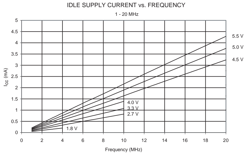
Figure 91. Idle Supply Current vs. Frequency (1 - 20 MHz)
