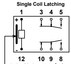
Index Mark on top of relay indicates position of pins 1 & 12 Pin Functions Bottom View
