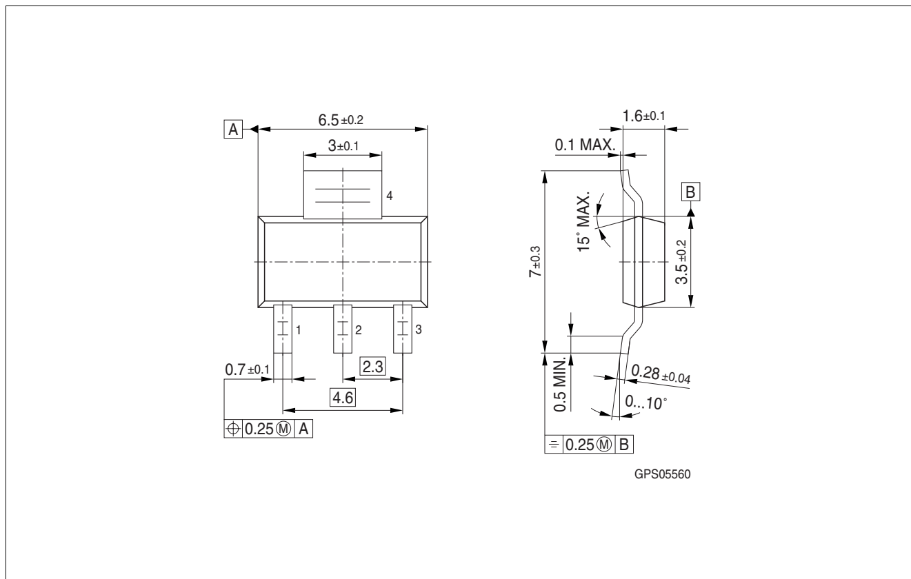
Figure 8 PG-SOT223-4
