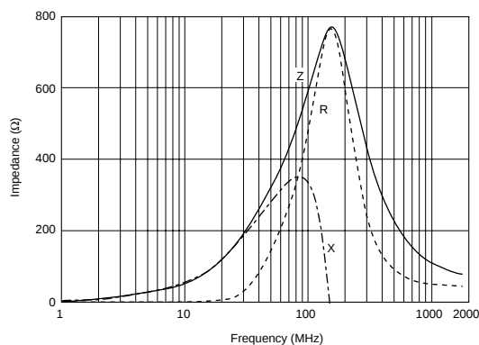
BLM31BE601FN1
