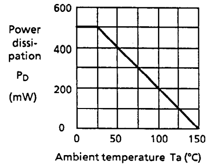
Figure 19 Package power dissipation (before mounting)
