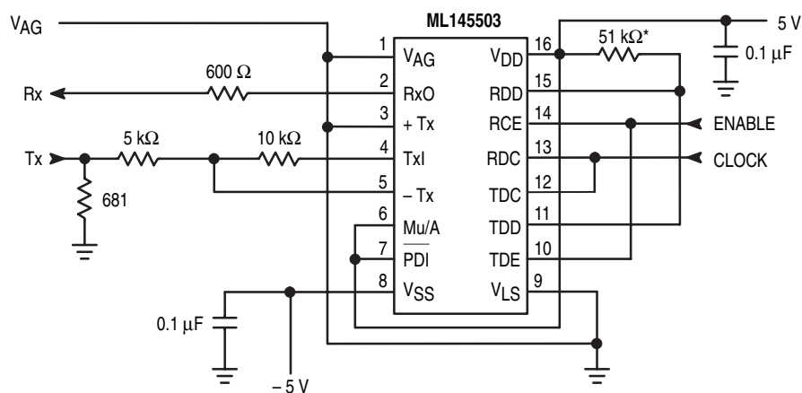
Figure 1. Test Circuit
