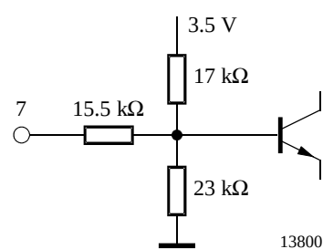
Figure 9. AGC switch (Pin 7)
