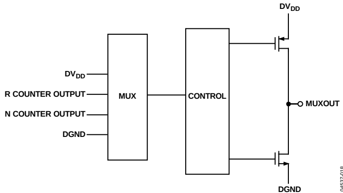
Figure 12. MUXOUT Circuit
