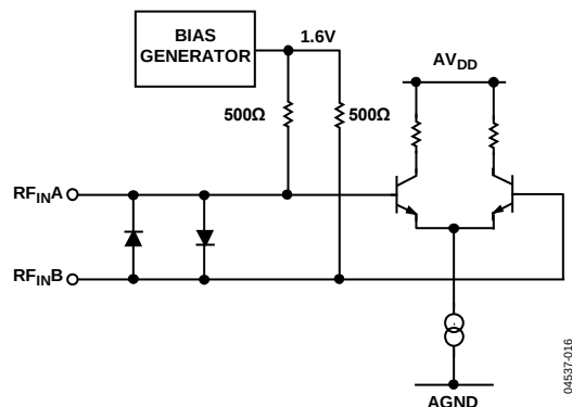
Figure 10. RF Input Stage
