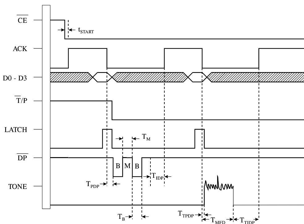
Figure 1. Switching diagram
