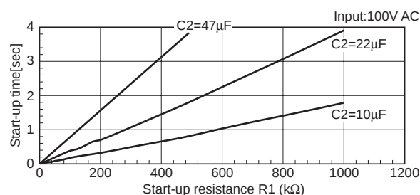
Fig. 5 Start-up time
