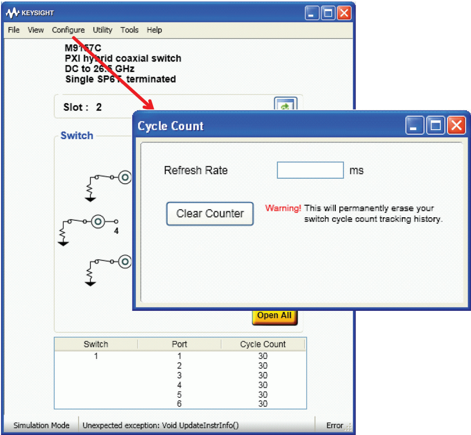
Figure 2. Onboard switch cycle count tracking eases maintenance and reduces unexpected system downtime.
