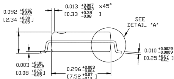
END VIEW
