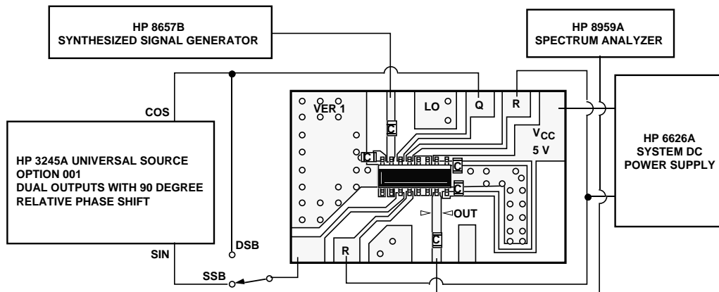
Figure 27. HPMX-2005 Single/Double Sideband Test Setup.
