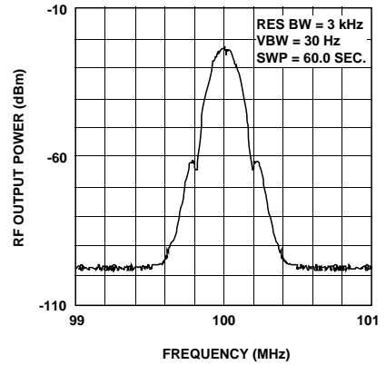
Figure 33. HPMX-2005 GSM Modulation Spectrum at 85^\circ\text{C} .
