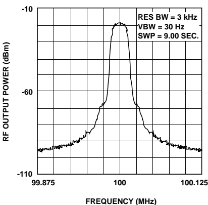
Figure 38. HPMX-2005 NADC Modulation Spectrum at 25^\circ\text{C} .
