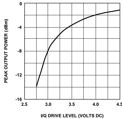
Figure 8. HPMX-2005 Power Output vs. I/Q Drive Level at 100 MHz. V_{CC} = 5\text{ V} , LO = -12\text{ dBm} , V_{Iref} = V_{Qref} = 2.5\text{ V} , V_{Imod} = V_{Qmod} = 3.25\text{ V} , T_A = 25^\circ\text{C} .
