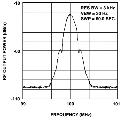
Figure 31. HPMX-2005 GSM Modulation Spectrum at -40^\circ\text{C} .
