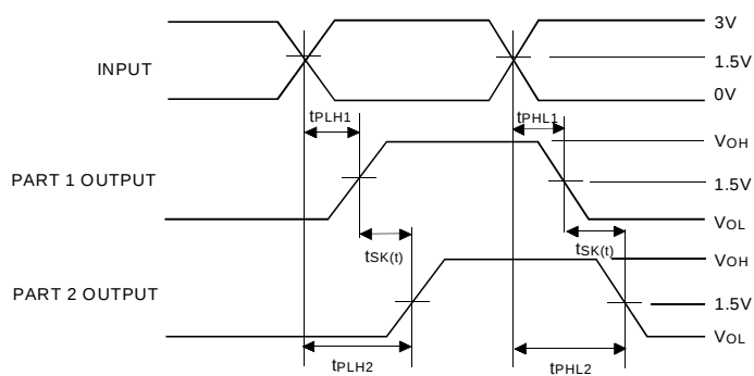
PART-TO-PART SKEW — t_{SK}(T)
