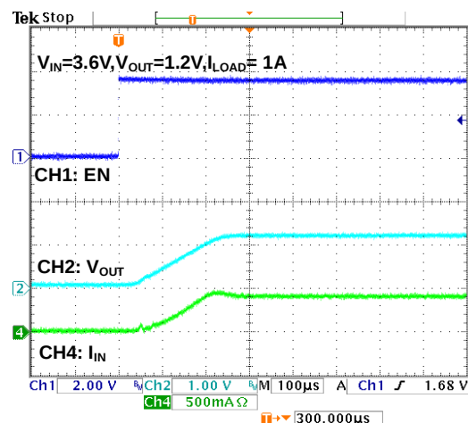
Figure 17. Start-up Waveform
