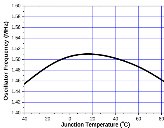
Figure 8. Frequency vs. Junction Temperature
