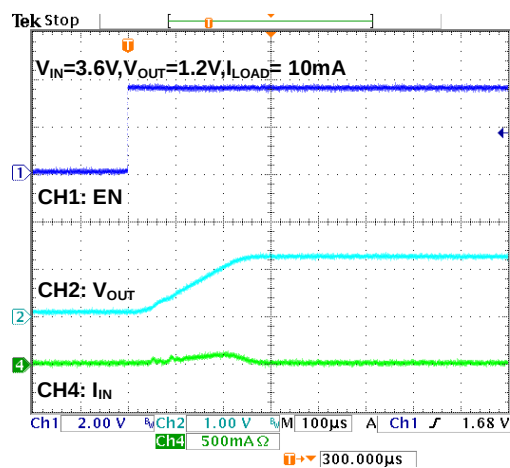
Figure 16. Start-up Waveform
