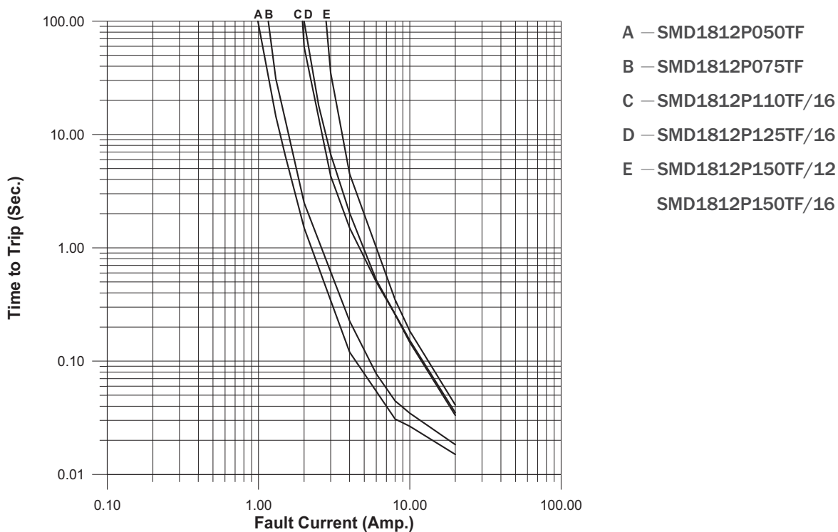
Average Time-Current Curve
