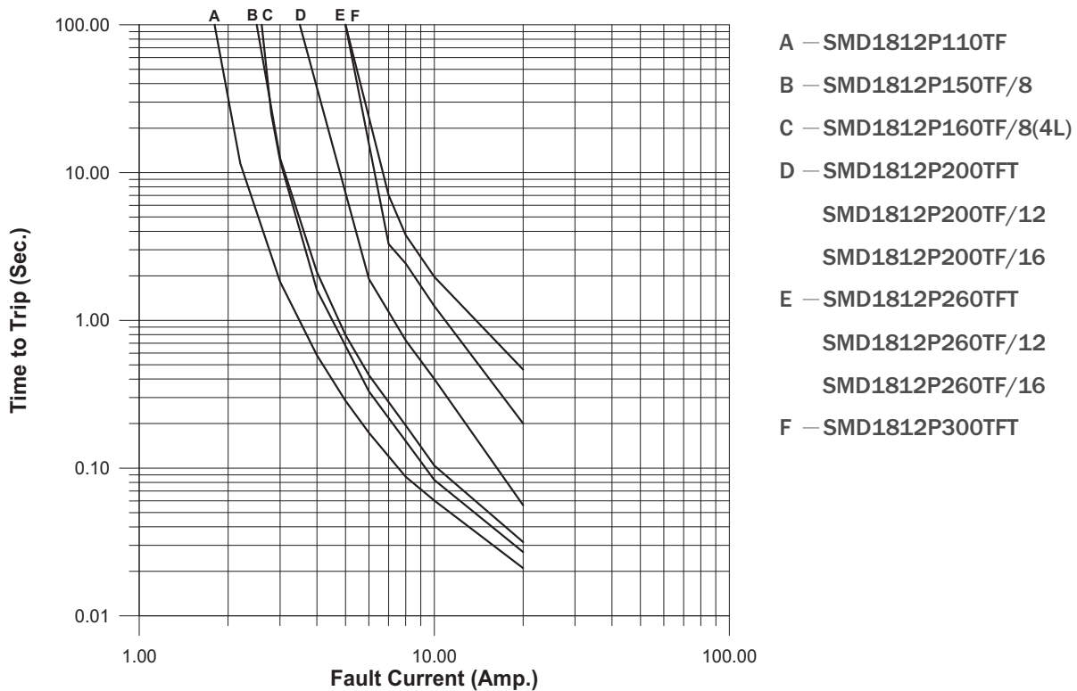
Average Time-Current Curve
