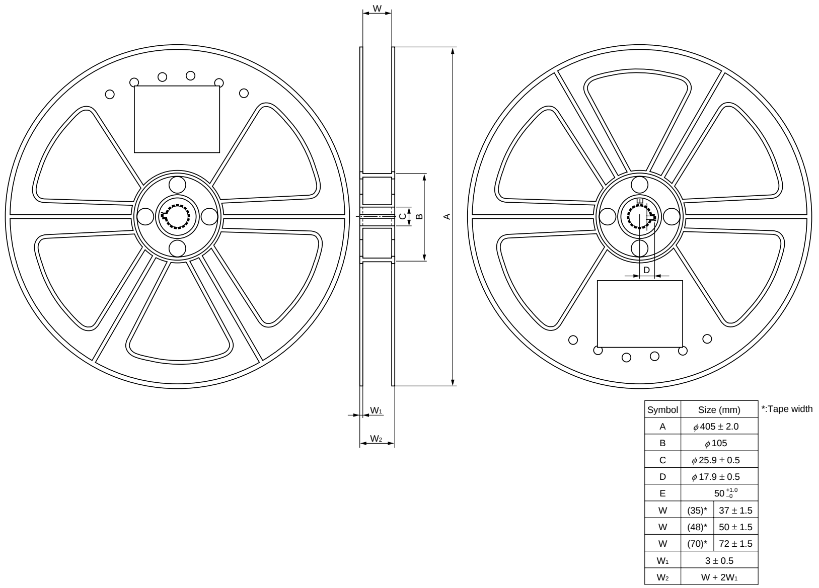
REFERENCE 2 : TCP SHIPPING REEL (φ 405 mm)
