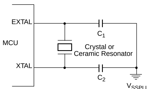
Figure 1-7. Loop Controlled Pierce Oscillator Connections ( \overline{\text{XCLKS}} = 1 )
