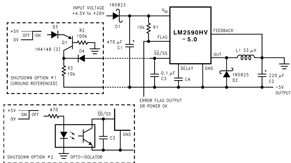
Figure 31. Inverting, -5-V Regulator With Shutdown and Soft-Start
