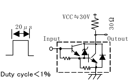
Figure 1. Switching Time Test Circuit & Timing Chart
