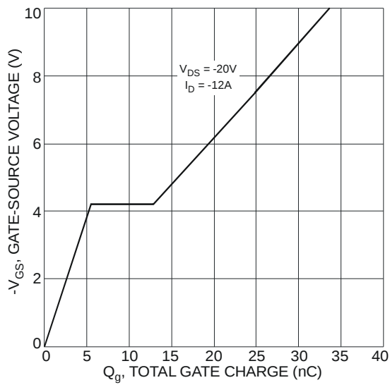
Fig. 13 Gate-Charge Characteristics
