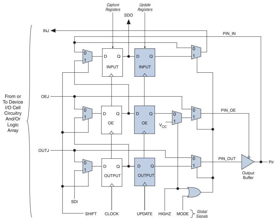
Figure 9–4. Stratix II and Stratix II GX Device's User I/O BSC with IEEE Std. 1149.1 BST Circuitry
