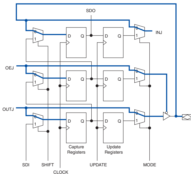
Figure 9–8. IEEE Std. 1149.1 BST SAMPLE/PRELOAD Mode
