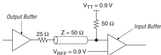
Figure 4–3. 1.8-V SSTL Class I Termination
