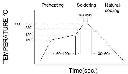
Figure 1. Re-flow Soldering
