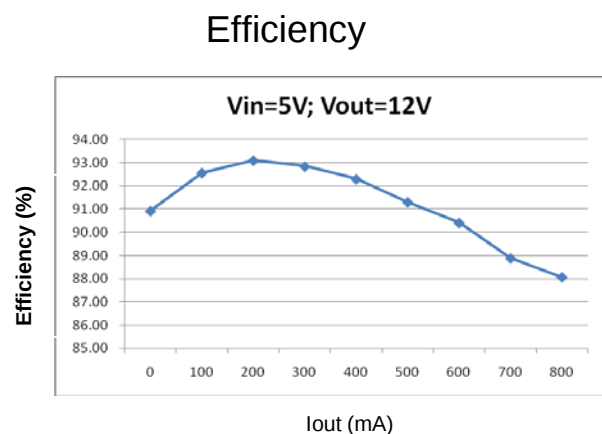
Figure 2. Efficiency Curve
