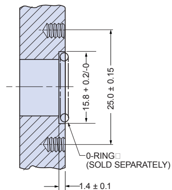
2 Panel cutout for Style B and F with O-ring VG96934Z2.
