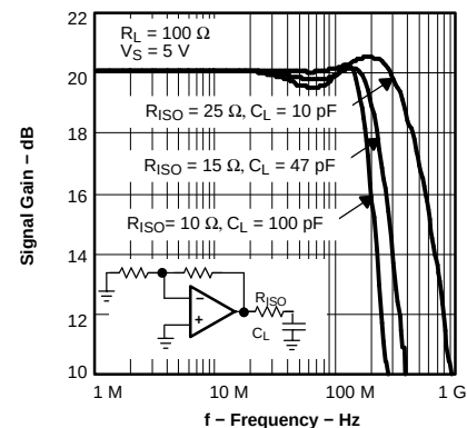
Figure 47. Driving Capacitive Loads
