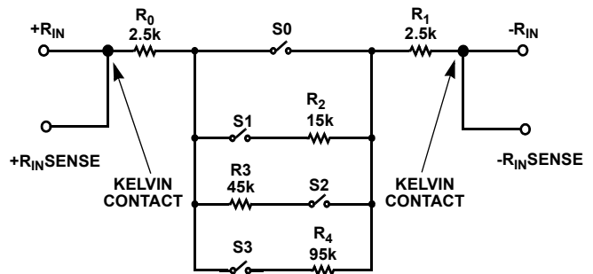
FIGURE 52. SWITCH EXAMPLE
