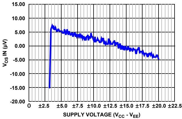
FIGURE 18. V_{OSIN} vs SUPPLY VOLTAGE
