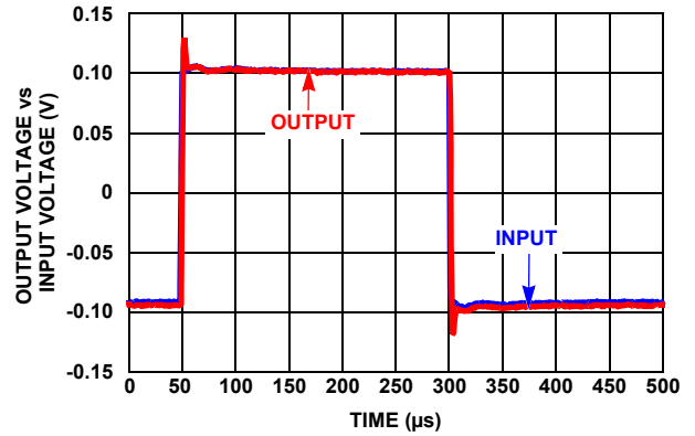
FIGURE 43. SMALL SIGNAL RESPONSE ( A_V = 1 , R_F = 30.1k )
