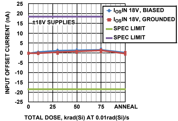
FIGURE 6. INPUT OFFSET CURRENT vs TOTAL DOSE
