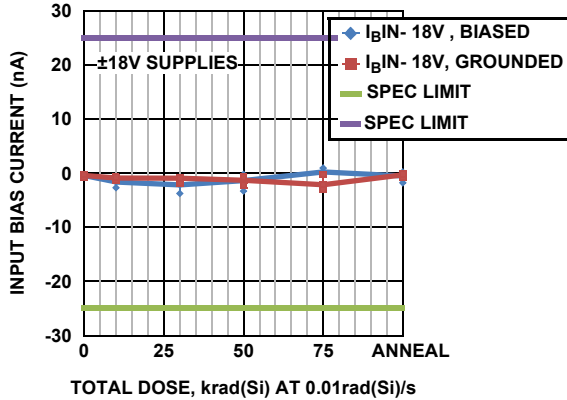
FIGURE 5. INPUT BIAS CURRENT I_{B\text{IN}-} vs TOTAL DOSE
