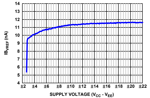
FIGURE 23. I_{BREF} vs SUPPLY VOLTAGE ( V_{CC} - V_{EE} )
