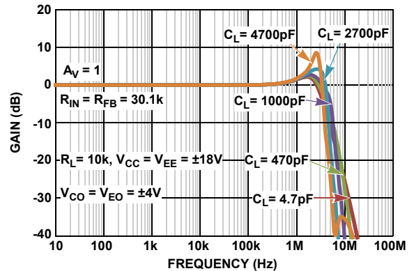
FIGURE 47. CLOSED LOOP GAIN vs FREQUENCY vs C_L
