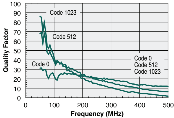
Quality Factor vs. Frequency DFN Package
