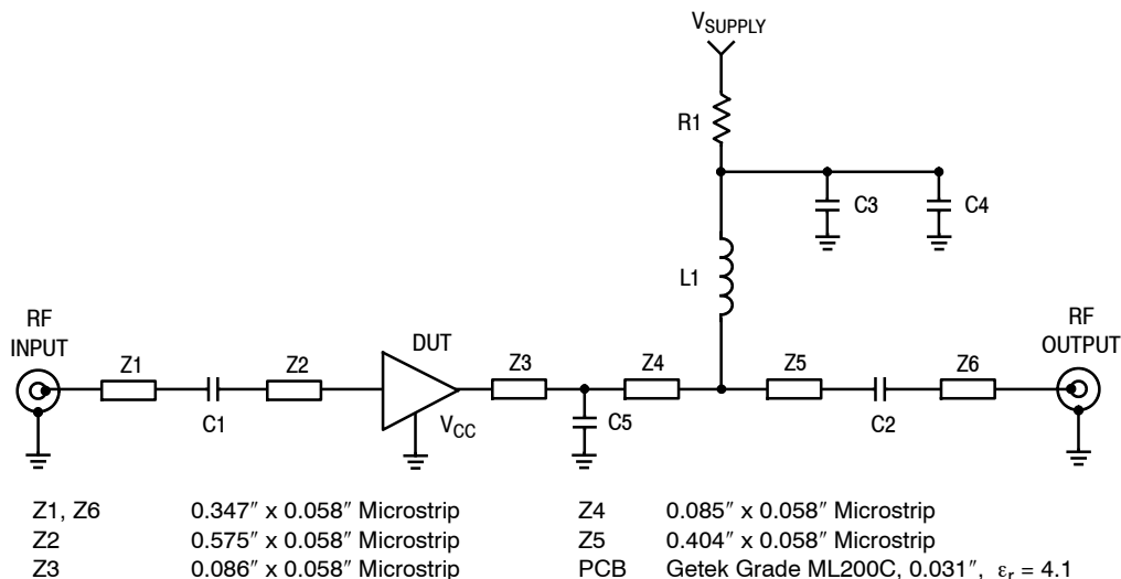
Figure 20. 50 Ohm Test Circuit Schematic
