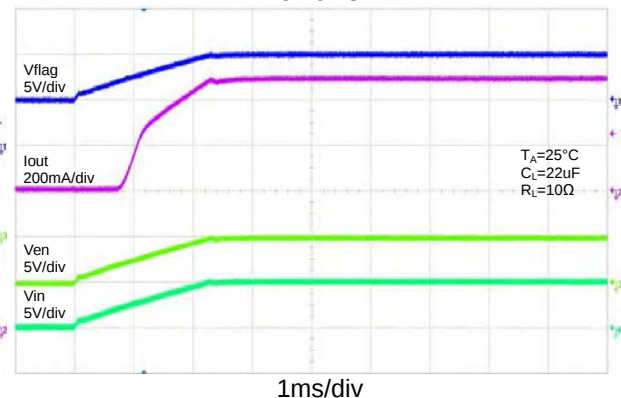
Power On
