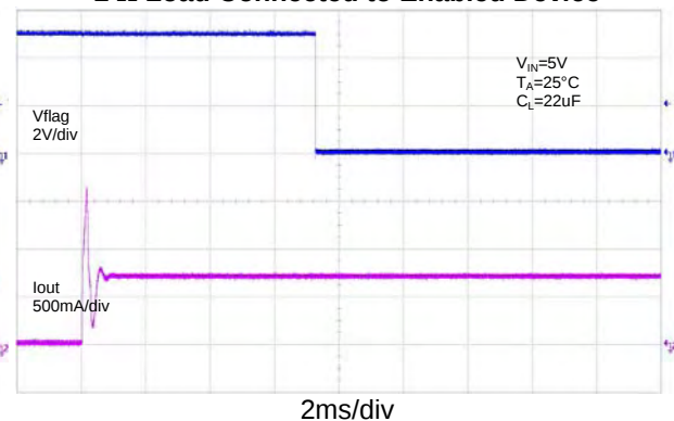
2 \Omega Load Connected to Enabled Device
