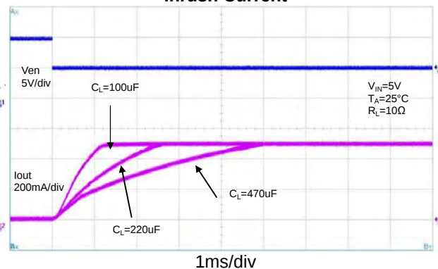
Inrush Current
