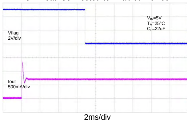
3 \Omega Load Connected to Enabled Device
