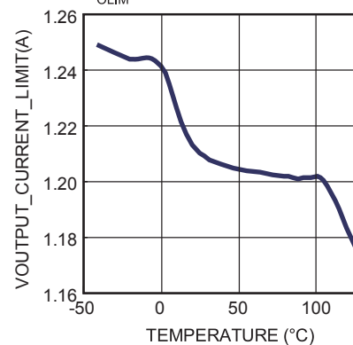
Output_Current_Limit_1.2A vs. Temperature
