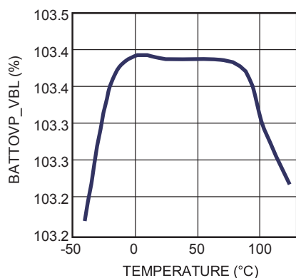
BATTOVP_VBL_% vs. Temperature
