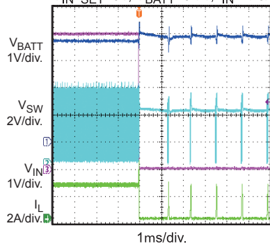
Boost Output Short Circuit Entry
