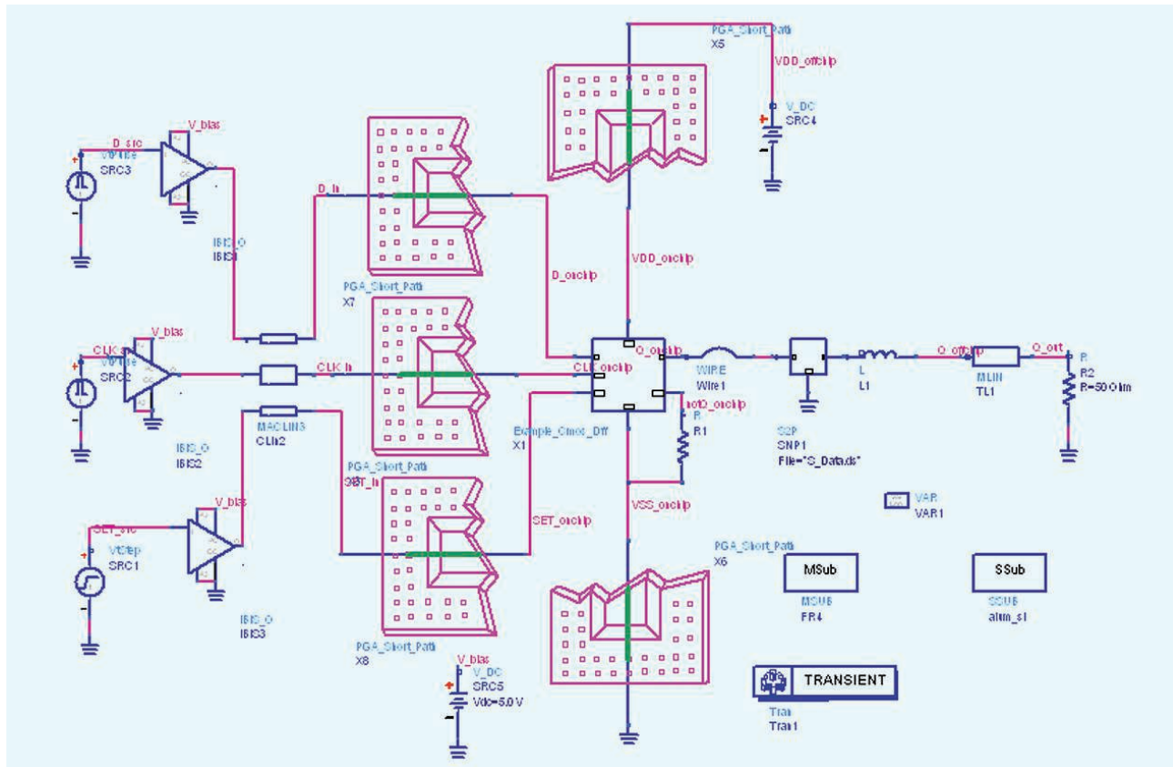
Figure 12. IBIS model palette and schematic showing time-domain simulation of IBIS models, package traces, and nonlinear transistor devices based on ASIC and S-parameter models.
