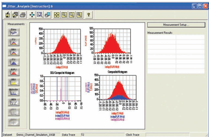
Figure 10. ADS provides powerful jitter analysis for analyzing all the random and deterministic jitter components present in a digital signal. It also provides accurate BER bathtub plots. The capability is based on patented EZJIT Plus technology, which is available in Keysight's real-time oscilloscopes.
