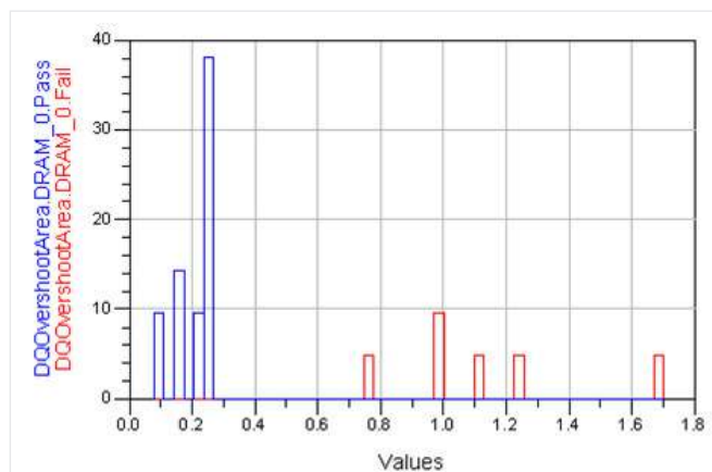
Figure 5. Pass-fail plot from the DDR3 compliance histogram measurements for DQ overshoot area
