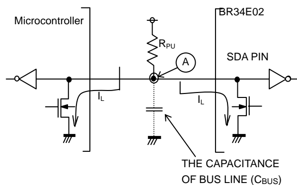
Figure 45. I/O Circuit
