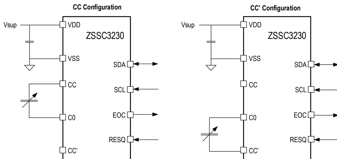
Figure 7. Capacitive Input in Differential Mode
