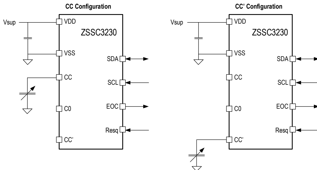
Figure 8. Capacitive Input in Single-Ended Mode
