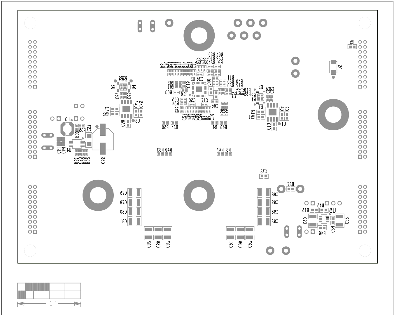
MAX15158Z EV Kit Component Placement Guide—Bottom Silkscreen
