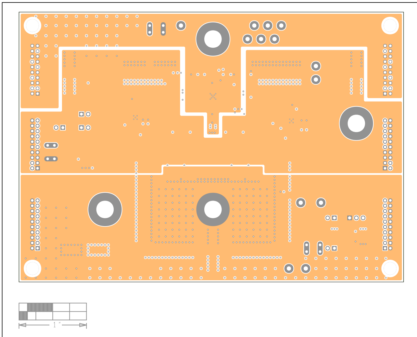
MAX15158Z EV Kit PCB Layout—Internal Layer 5
