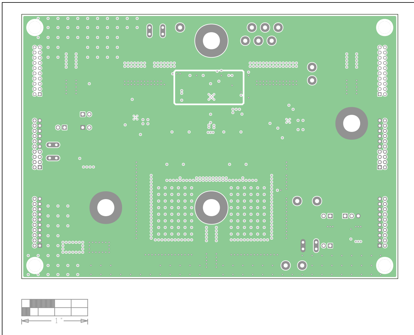
MAX15158Z EV Kit PCB Layout—Internal Layer 3
