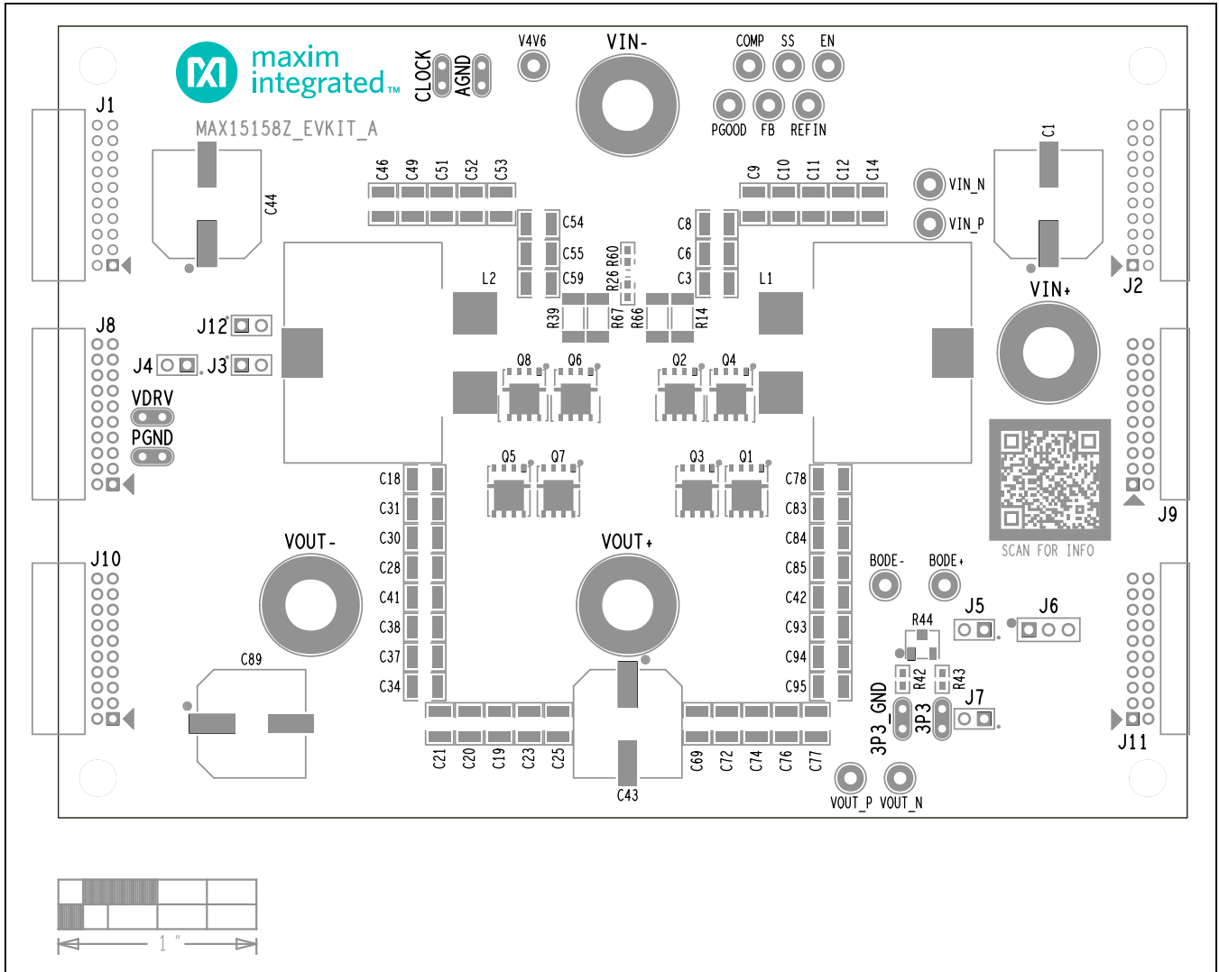
MAX15158Z EV Kit Component Placement Guide—Top Silkscreen
