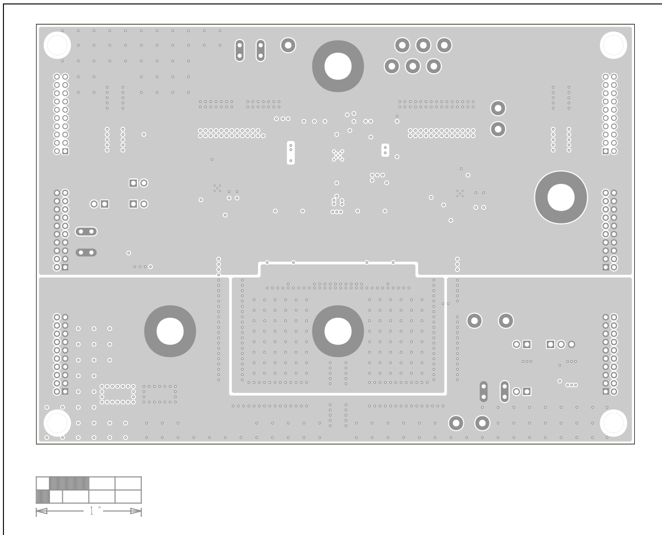
MAX15158Z EV Kit PCB Layout—Internal Layer 2
