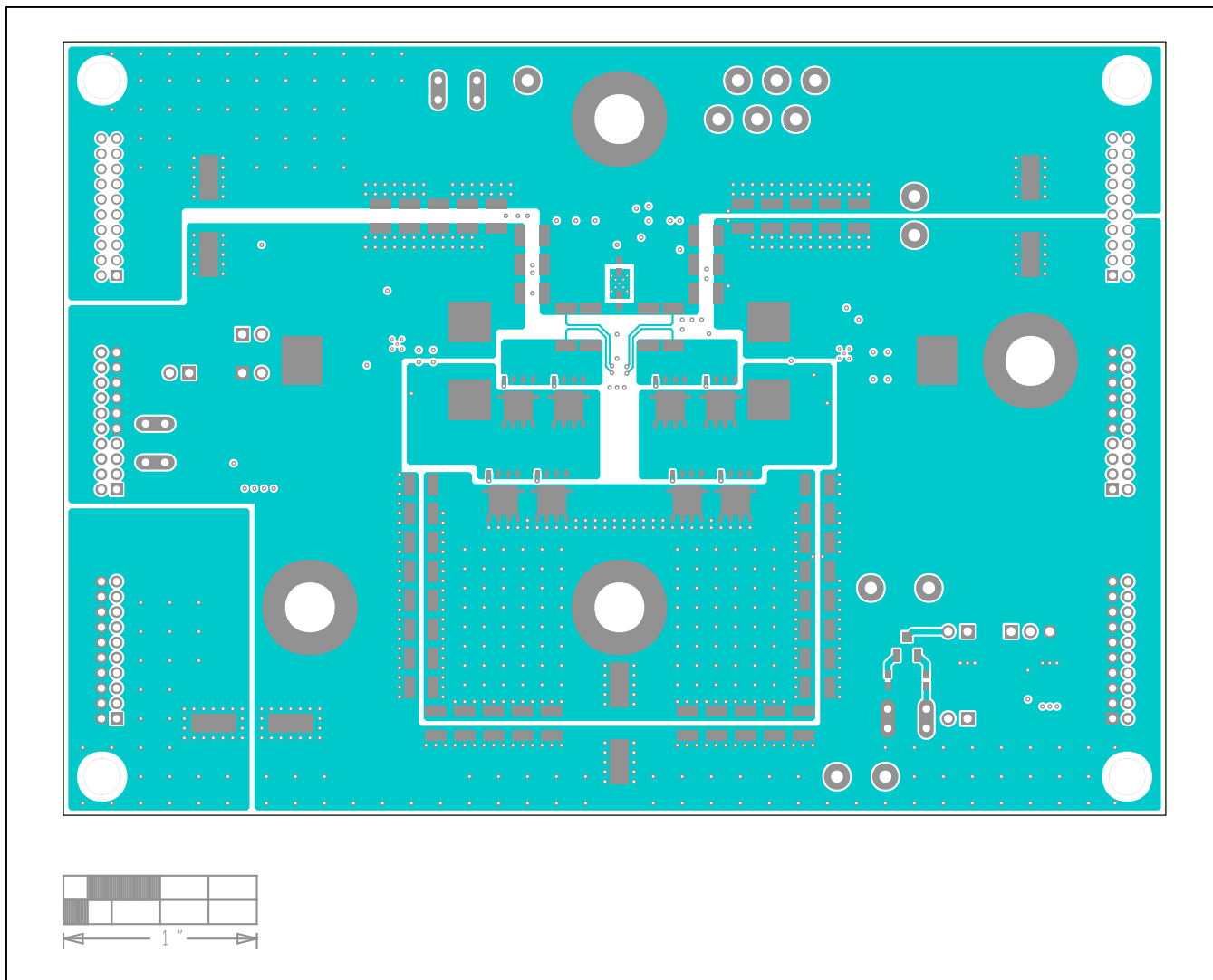
MAX15158Z EV Kit PCB Layout—Top Layer
