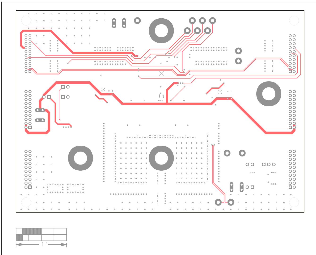
MAX15158Z EV Kit PCB Layout—Internal Layer 4
