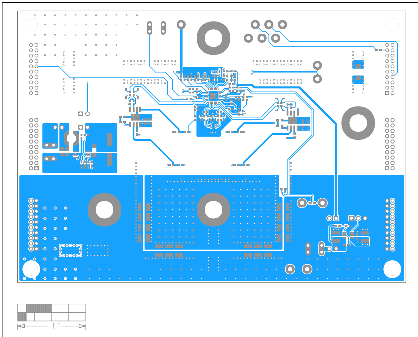
MAX15158Z EV Kit PCB Layout—Bottom Layer
