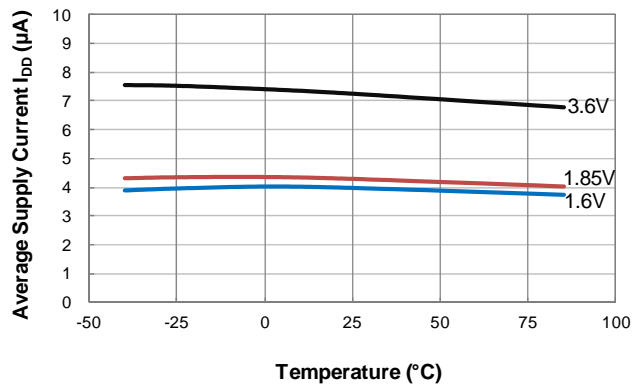
Average Supply Current vs. Temperature
