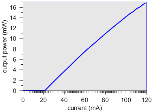
Current-Output-Power
