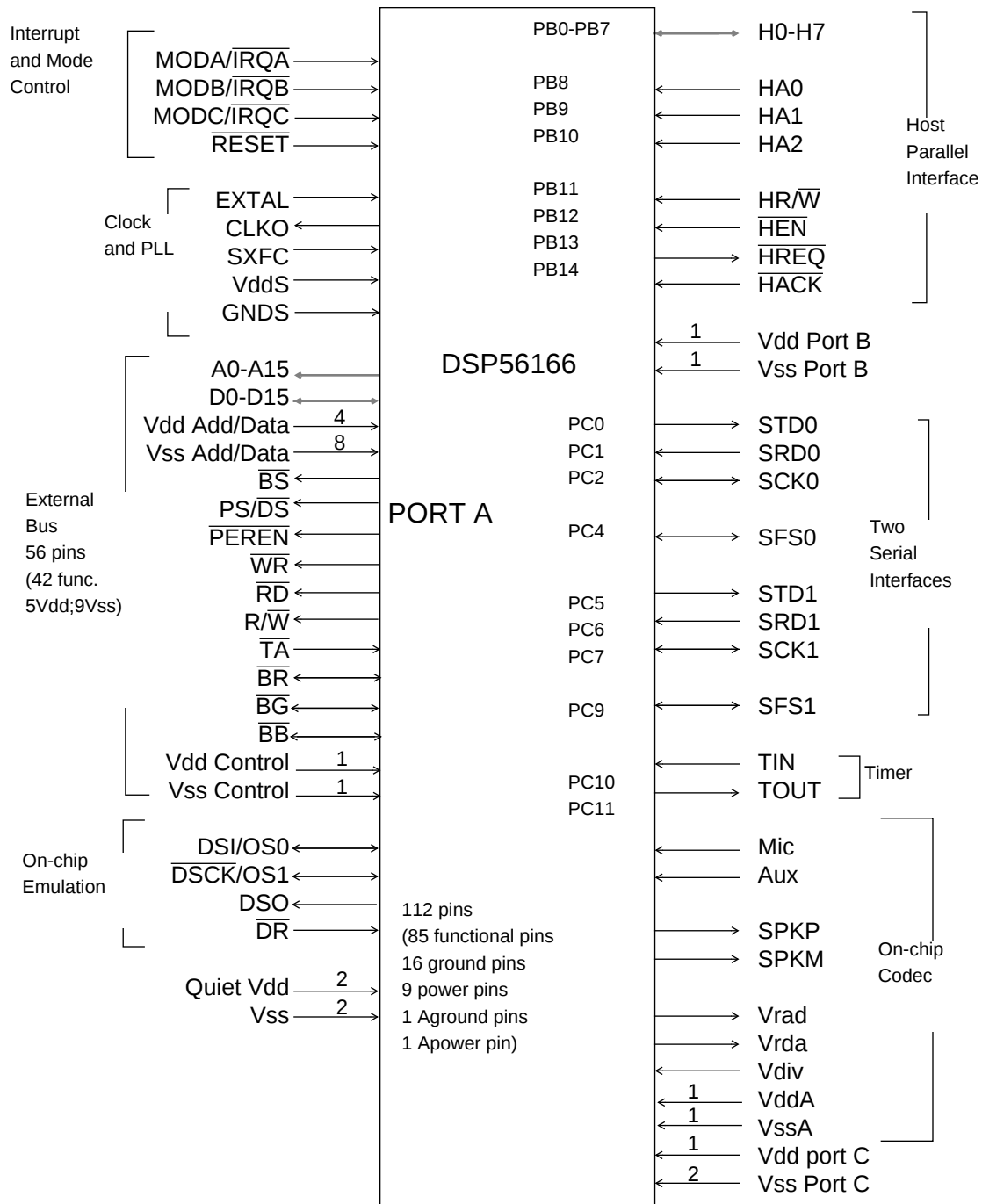
Figure 3 DSP56166 Pinout
