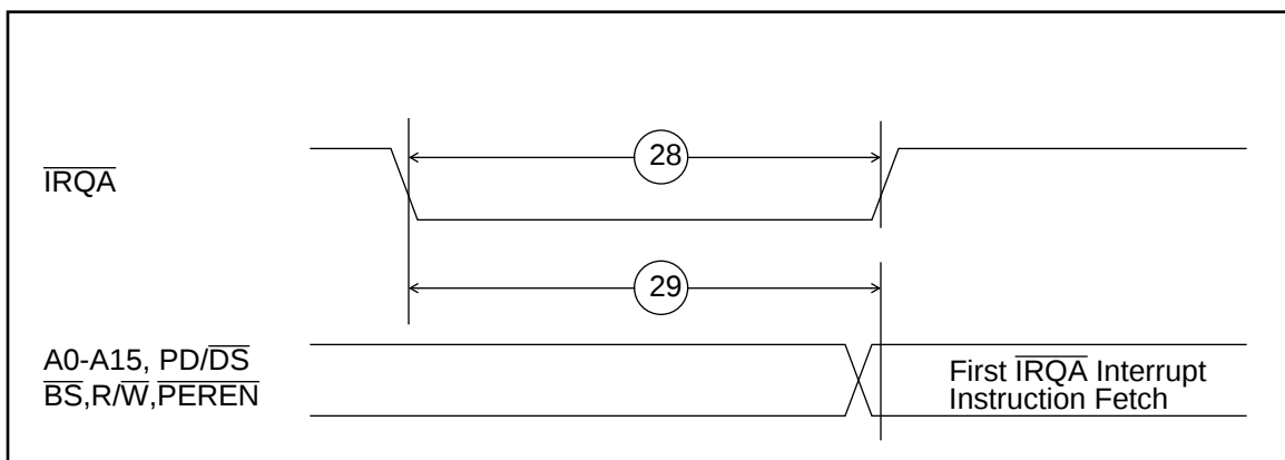
Wait and Stop 3. Recovery from Stop State Using \overline{\text{IRQA}} Interrupt Service
