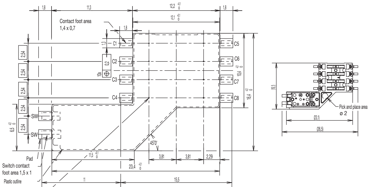
RECOMMENDED PC BOARD LAYOUT (Component side)
