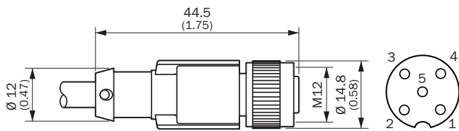
female connector M12 x1, straight, screened
