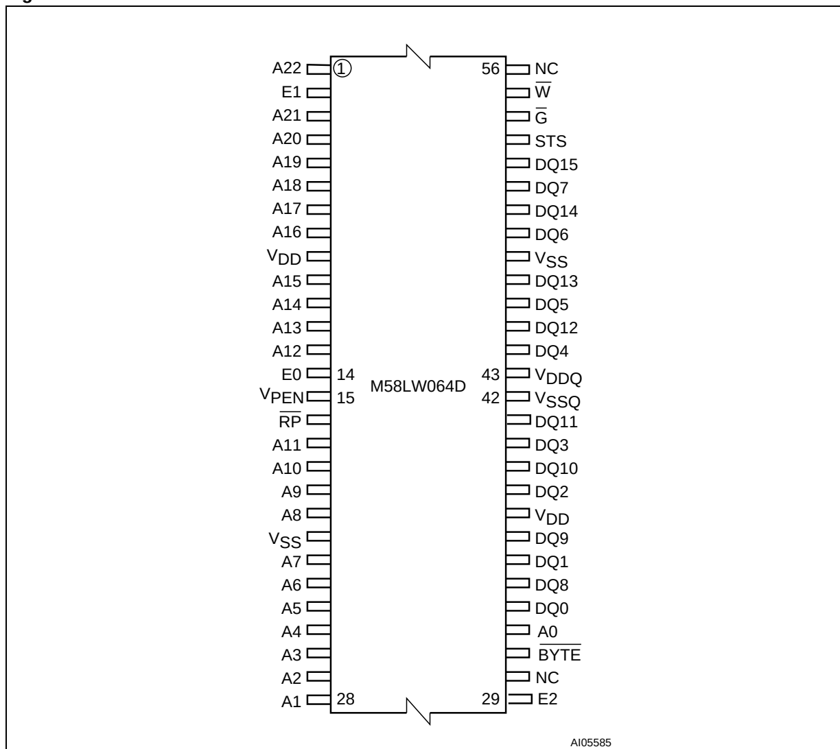
Figure 3. TSOP56 Connections
