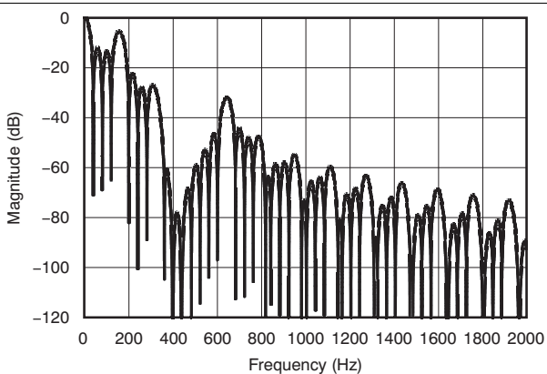
Figure 61. Filter Profile with Data Rate = 40 SPS
