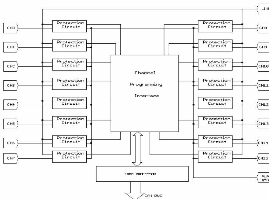
Figure 1 – Block Diagram
