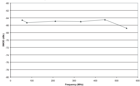
Figure 11: XMOD vs. Frequency
