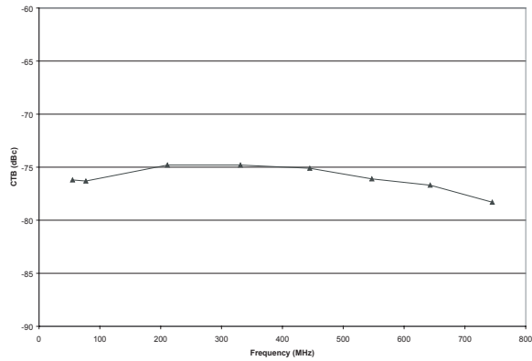
Figure 12: CTB vs. Frequency (V DD = +12 V, I DD = 195 mA, 112 Analog Channels, 3 dB Tilt, +37 dBmV output power at 1 GHz)
