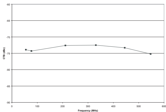
Figure 9: CTB vs. Frequency
