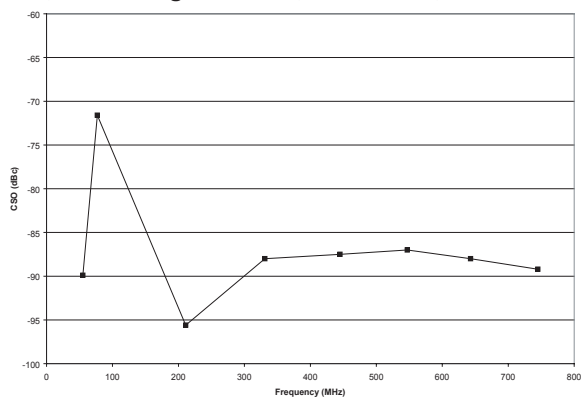
Figure 24: CSO vs. Frequency
