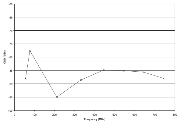
Figure 13: CSO vs. Frequency (V DD = +12 V, I DD = 195 mA, 112 Analog Channels, 3 dB Tilt, +37 dBmV output power at 1 GHz)
