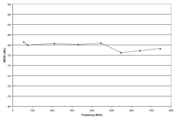
Figure 14: XMOD vs. Frequency (V DD = +12 V, I DD = 195 mA, 112 Analog Channels, 3 dB Tilt, +37 dBmV output power at 1 GHz)
