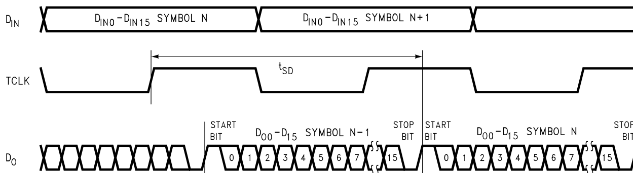
Figure 10. Serializer Delay
